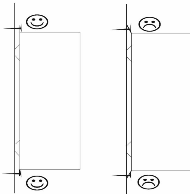
Side view of mounted panels
